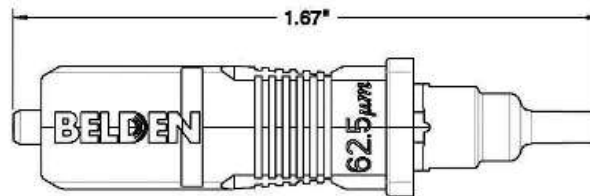
900 \mu\text{m} VERSION (OM1 SHOWN)
