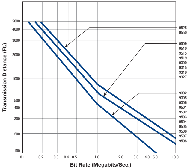
Bit Rate
