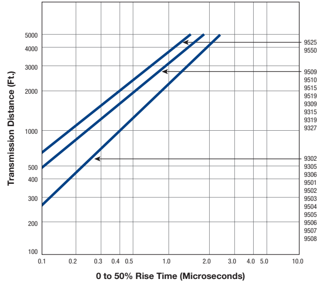
Rise Time
